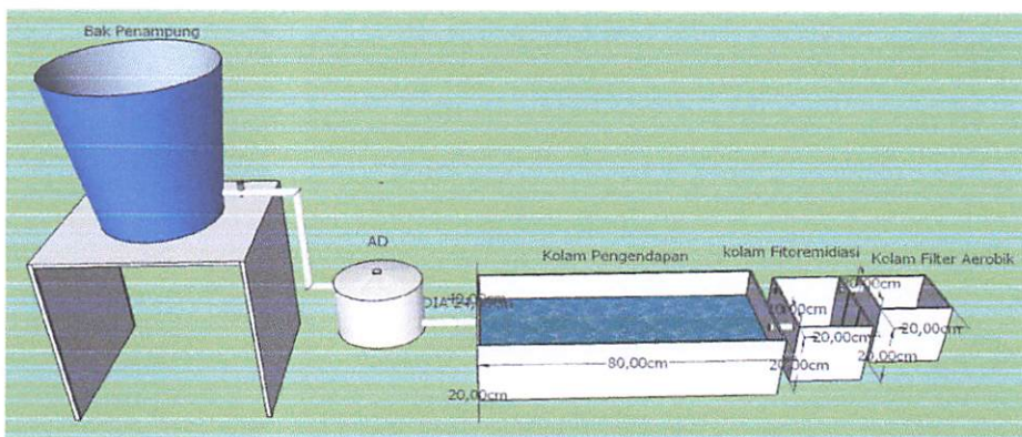
Gambar 3.1. Pilot Plant MCK PLUS Tlogomas
