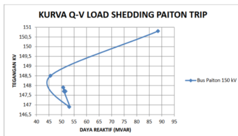
Gambar 18. Kurva Q-V Bus Paiton 150 kV Load Shedding
