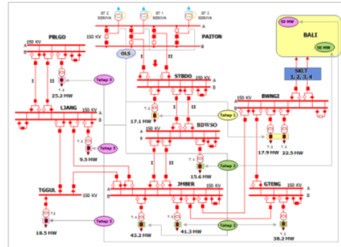
Gambar 8. Skema Load Shedding
