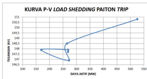
Gambar 16. Kurva P-V Bus Paiton 150 kV Load Shedding
