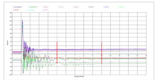
Gambar 6. Respon Sudut Rotor Gangguan Short Circuit
