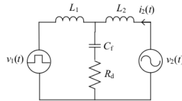
Fig. 4. LCL filter and its parameter.
