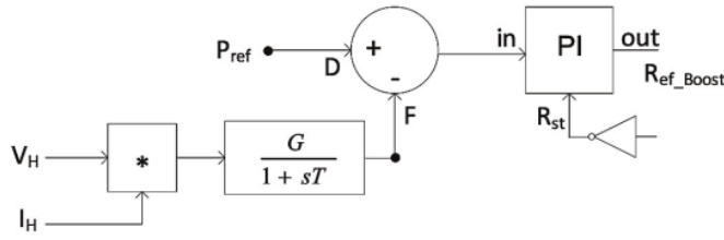
Fig. 3. Power controller.
