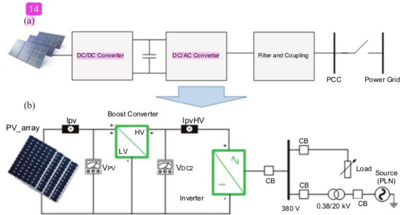
Fig. 1. Grid-connected PV system with a two-stage converter.
