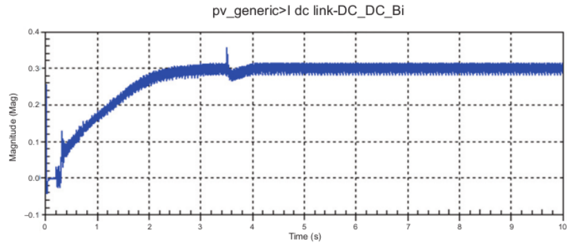
Fig. 10. DC power of the boost converter.
