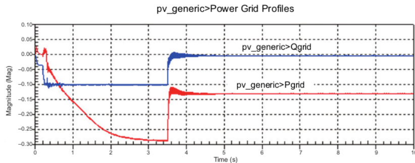
Fig. 13. Power grid profiles of the system.
