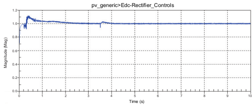
Fig. 9. DC current of the boost converter.
