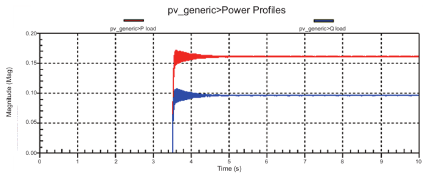
Fig. 11. The load power profiles.
