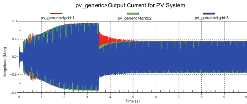
Fig. 14. Current grid profiles.
