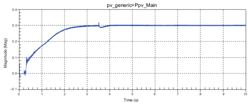
Fig. 8. DC voltage of the boost converter.
