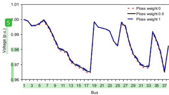
Fig. 3. Voltage profiles with different weights considering optimal power factor.
