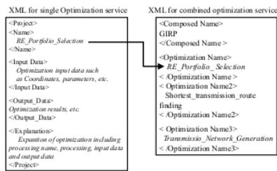
Fig. 5. XML texts of metadata for optimization
