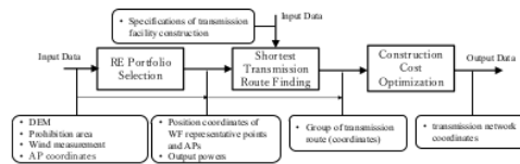
Fig. 7. GIRP optimization process
