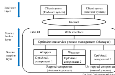
Fig. 2. GGOD architecture
