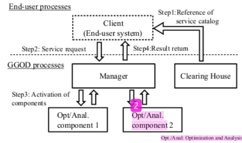
Fig. 3. Request and processing flows in GGOD
