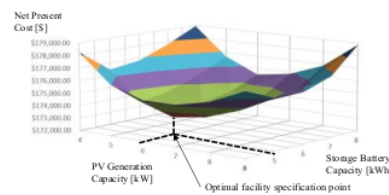
Fig. 11 Results of facility planning for single micro-grid
