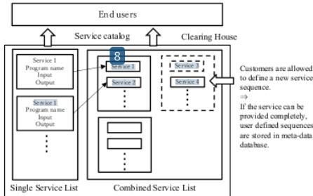
Fig. 4. Clearing house for optimization service
