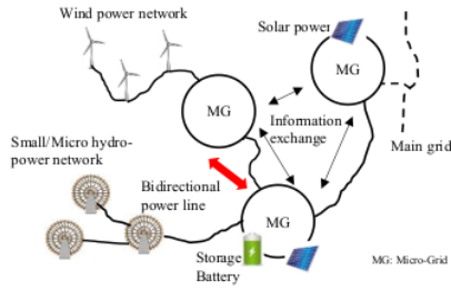
Fig. 1. Expandable micro-grid cluster
