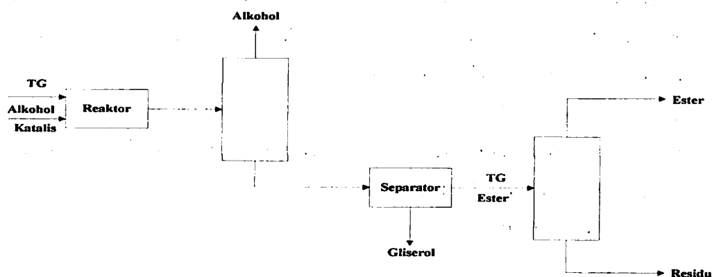
Gambar 2.2 Proses Henkel
