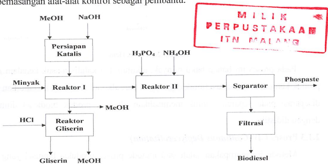
Gambar. 2.1. Proses Batchwise
