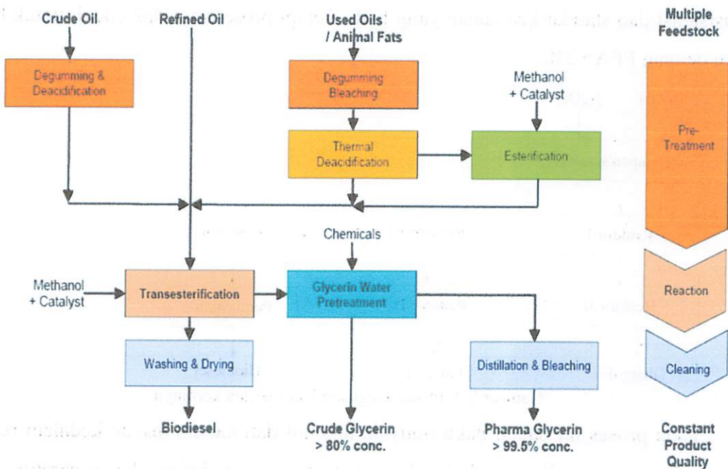
Gambar 2.4. Proses Lurgi
