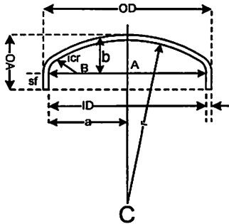
Gambar 6.3. tutup atas standard dished
