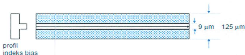
Gambar 2.6 : Step Index Single Mode
