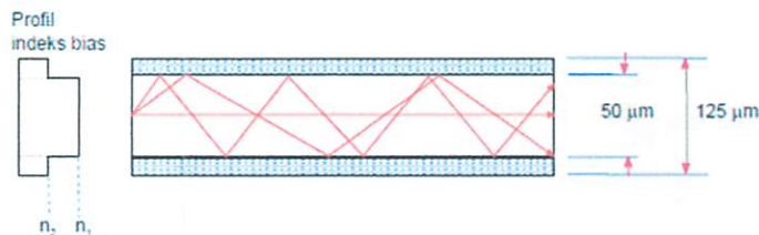
Gambar 2.4 : Step Index Multi Mode
