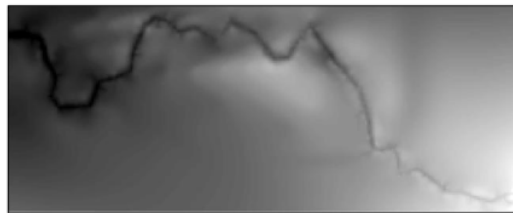
Gambar 3. Digital Elevation Modelling (DEM)
