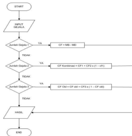
Gambar 5 Flowchart Metode Certainty Factor
