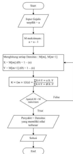
Gambar 4 Flowchart Metode Dempster Shafer
