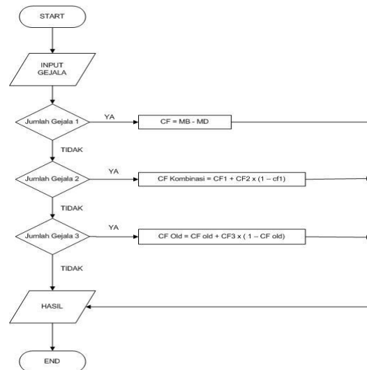
Gambar 5 Flowchart Metode Certainty Factor
