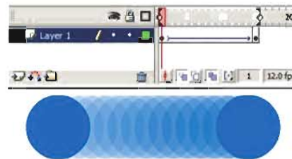
Gambar 3 Motion Tween .
