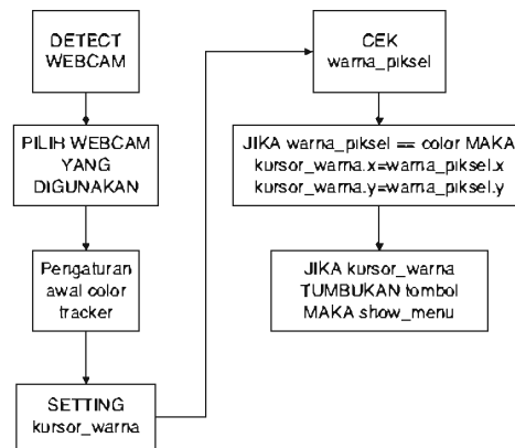
Gambar 7. Diagram Blok Color Tracker
