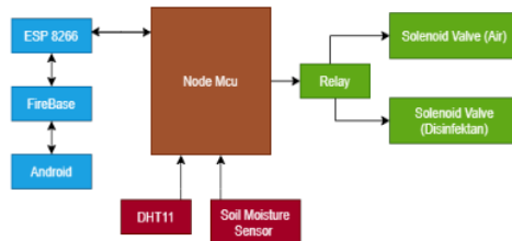
Gambar 6. Blok Diagram
