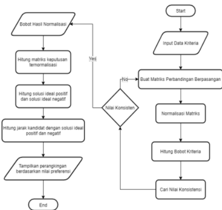
Gambar 4. Flowchart Metode
