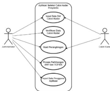
Gambar 5. Use Case Diagram
