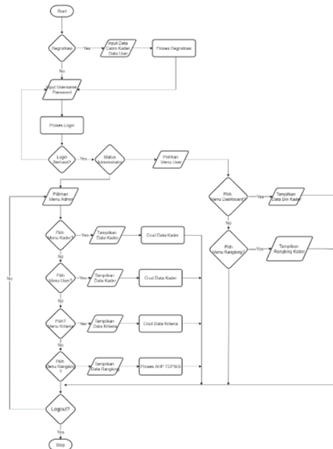
Gambar 3. Flowchart Sistem
