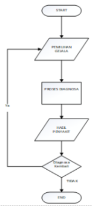
Gambar 3 Flowchart Sistem
