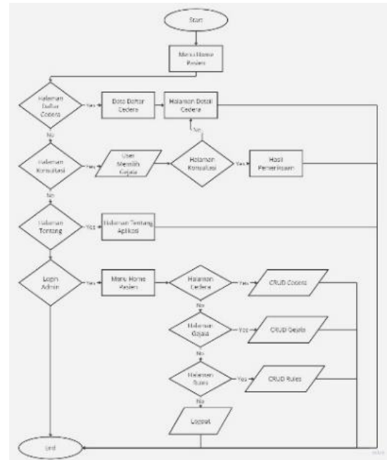
Gambar 4 Flowchart
