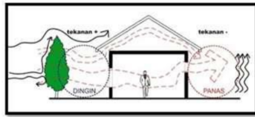
Gambar 18 cross ventilation
