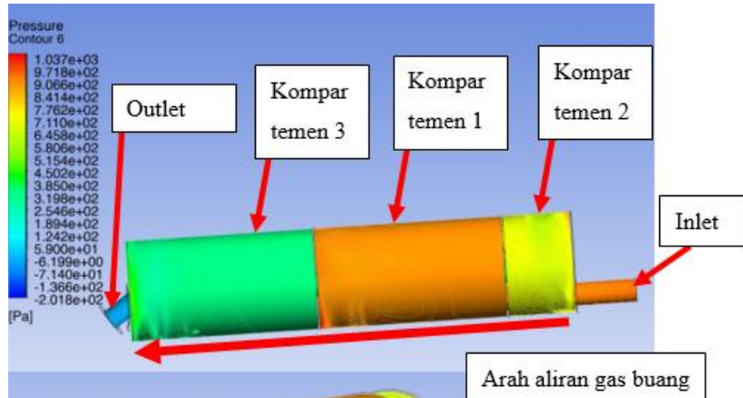
Gambar 5. Pressure Contour Muffler 1
