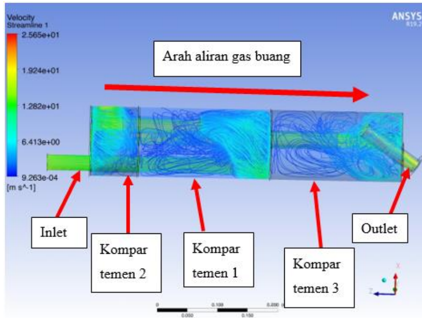
Gambar 2. Velocity Streamline Muffler 1
