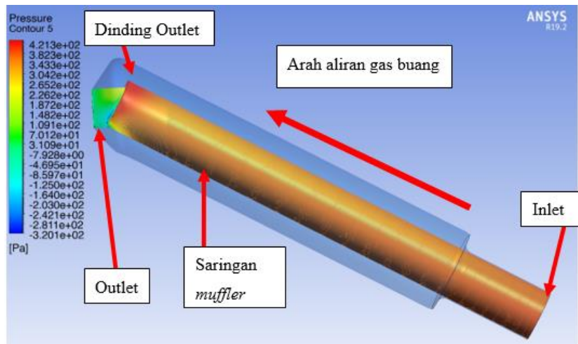
Gambar 6. Pressure Contour Muffler 2
