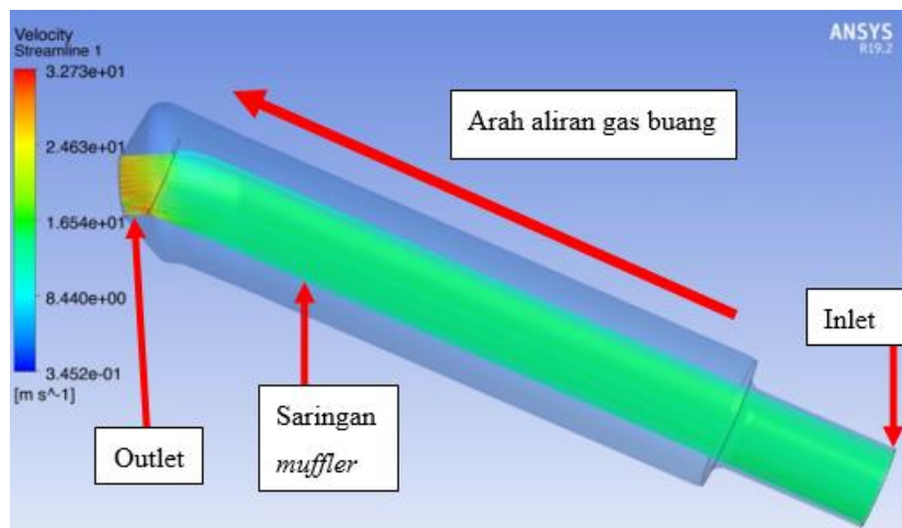
Gambar 3. Velocity Streamline Muffler 2
