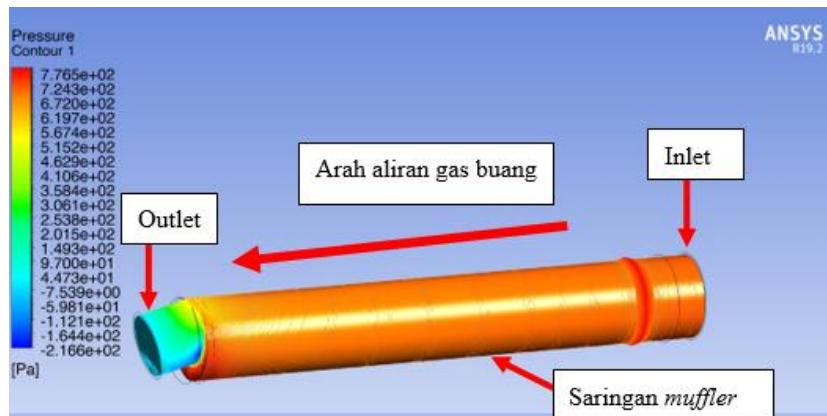
Gambar 7. Pressure Contour Muffler 3
