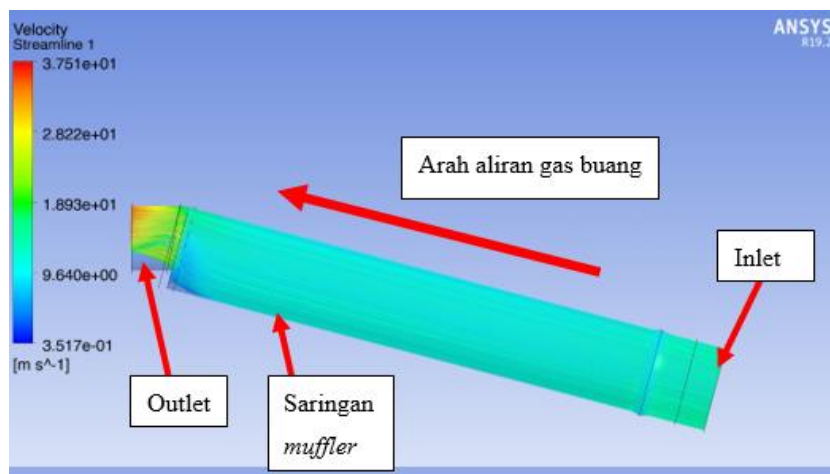
Gambar 4. Velocity Streamline Muffler 3
