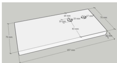
Gambar 6. Base plate
