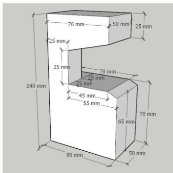
Gambar 1. Fixed Grip
