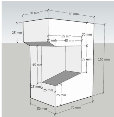
Gambar 2. Moving grip
