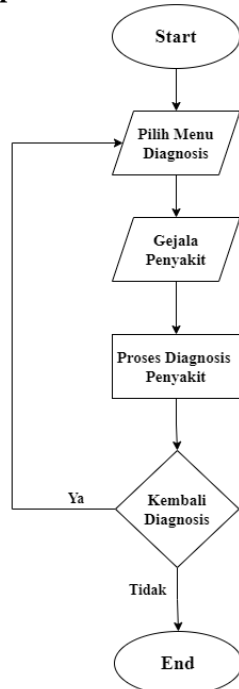
Gambar 4. Flowchart Sistem
