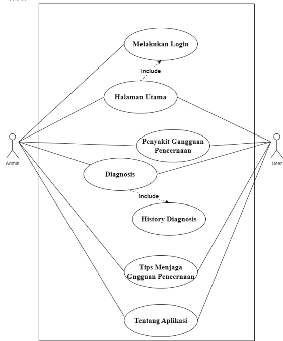
Gambar 6. Use Case
