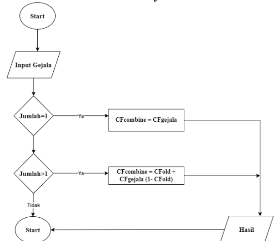
Gambar 5. Flowchart Metode Certainty Factor
