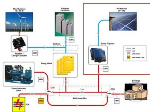
Gambar. 9 Single line diagram PLTS
