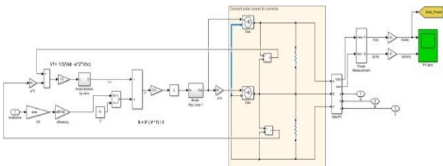
Gambar. 2 model Simulink PV
