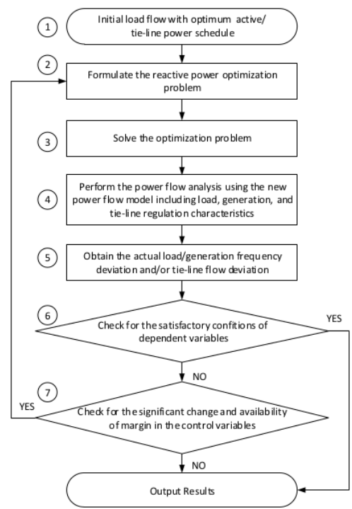
Figure 1. Flow chart of the algorithm for reactive power optimization in Large Inter-connected Power systems.
