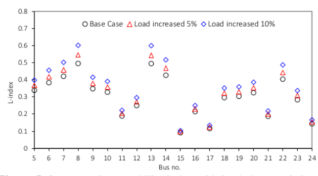
Figure 5. System voltage stability index with load characteristics.
