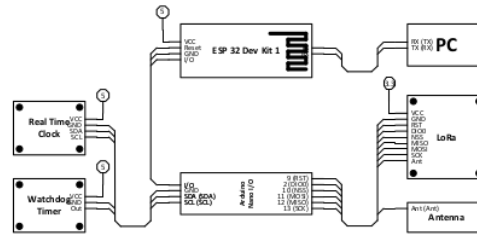
Gambar 3 Wiring Diagram Sink Node
