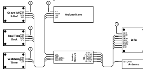
Gambar 2 Wiring Diagram Sensor Node
