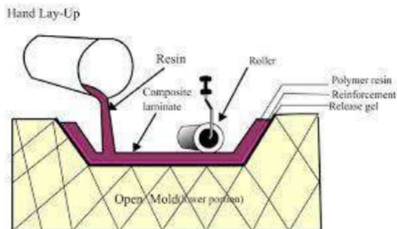
Gambar 3.1 Proses 2 Hand Lay Up
