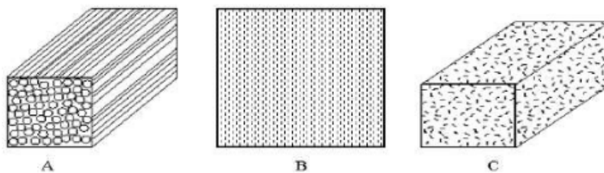
Gambar 1.3 Macam – macam komposit fiber (A. Continous/Long fiber B. Discontinous/short fiber aligned C. Discontinous/short fiber random )
