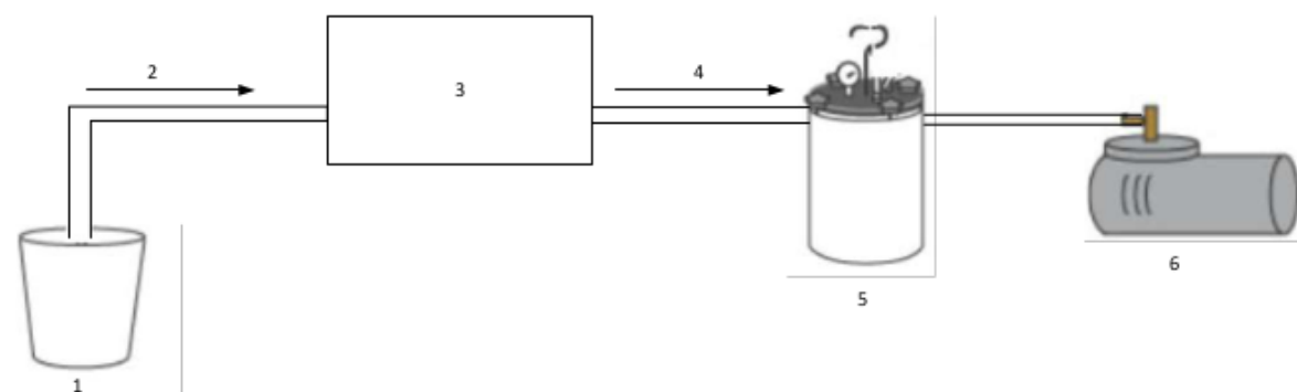
Gambar 3.2 Skema Vacuum Infusion Resin
