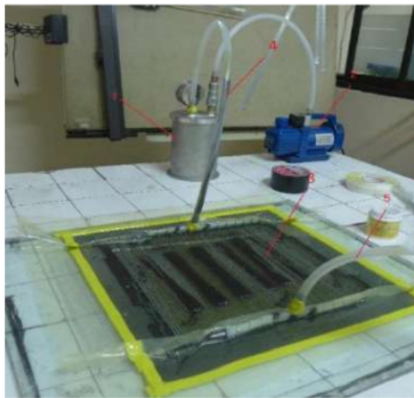
Gambar 5.3 Instalasi Vacuum Infusion Resin
