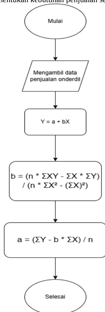
Gambar 1. Flowchart metode trend moment
