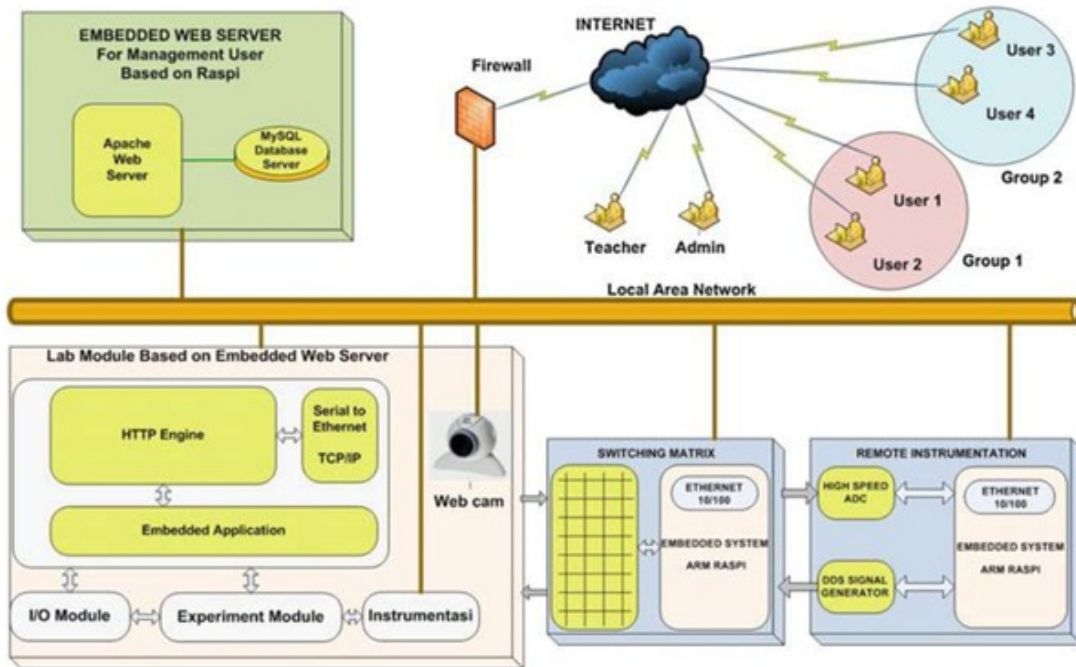
Fig. 60.1 Diagram of the remote lab architecture
