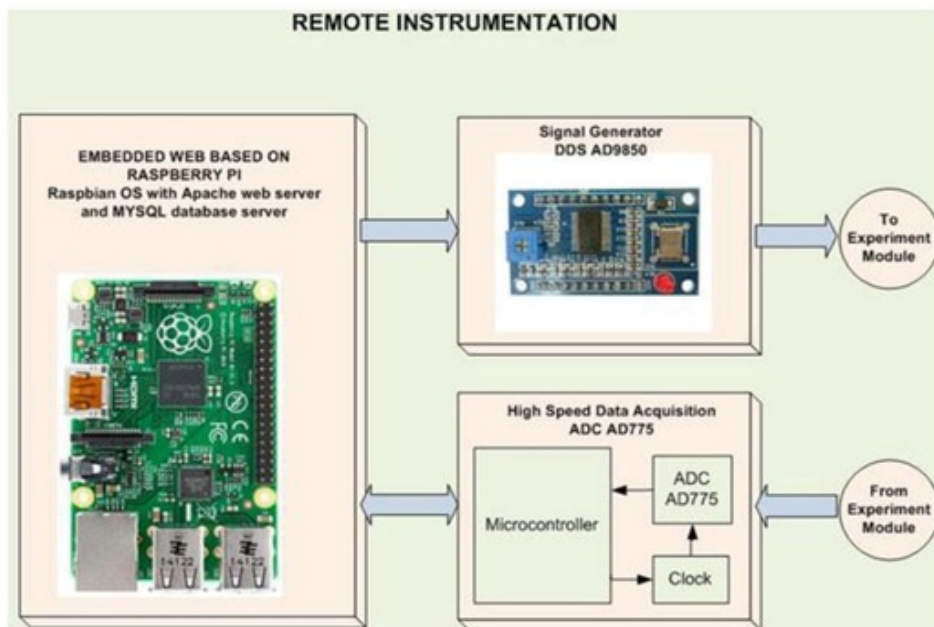
Fig. 60.2 Diagram of the remote instrumentations
