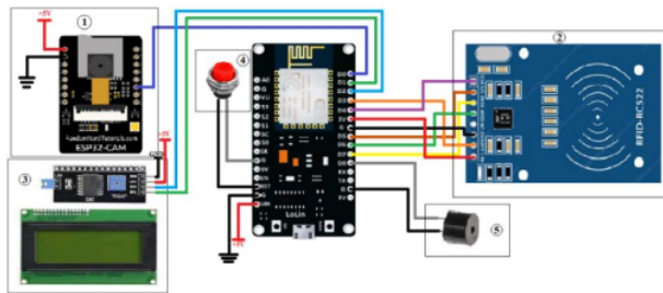
Gambar 5. Wiring Diagram
