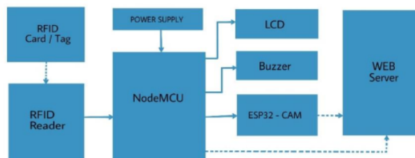
Gambar 4. Blok Diagram
