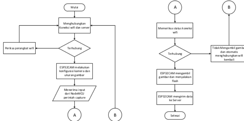
Gambar 7. Flowchart ESP32-CAM
