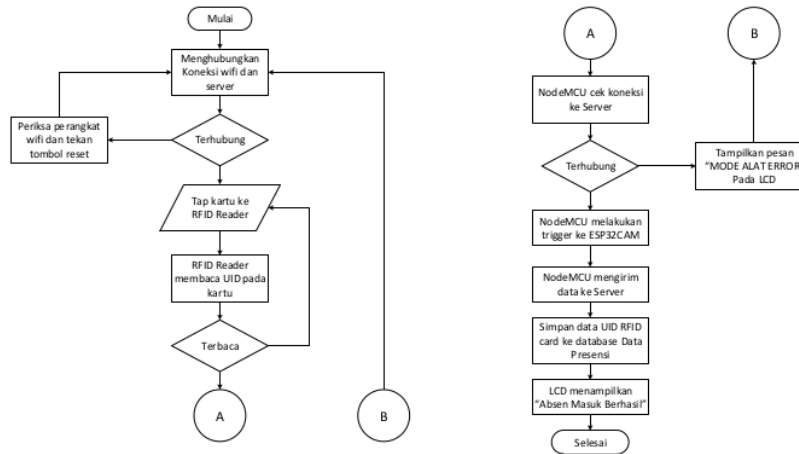
Gambar 6. Flowchart NodeMCU ESP8266
