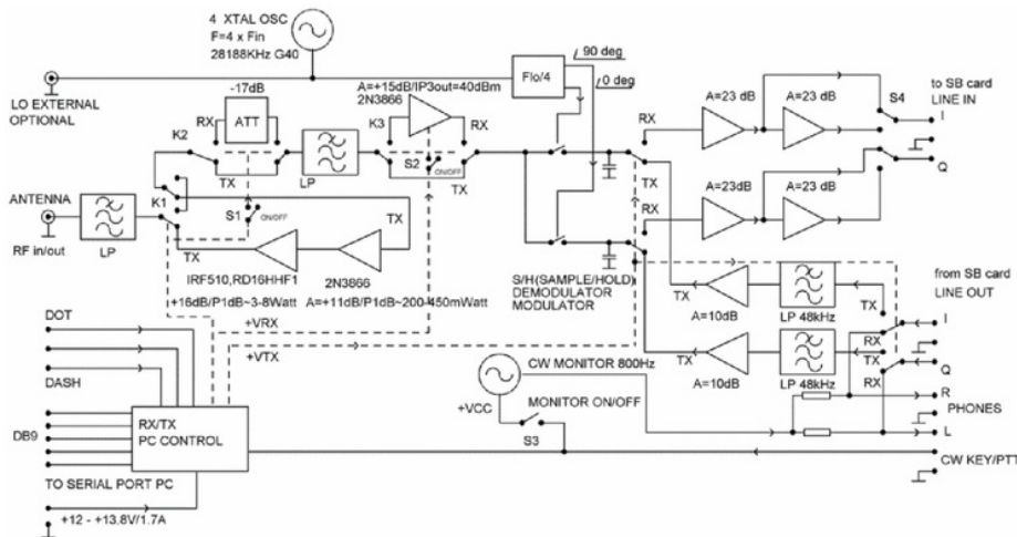
Gambar 2.3 Desain Transceiver SDR
