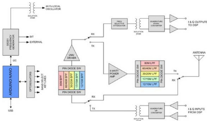
Gambar 3.1 Blok Diagram Sistem Low Noise SDR
