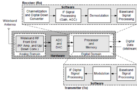
Gambar 2.2 Arsitektur Transceiver SDR
