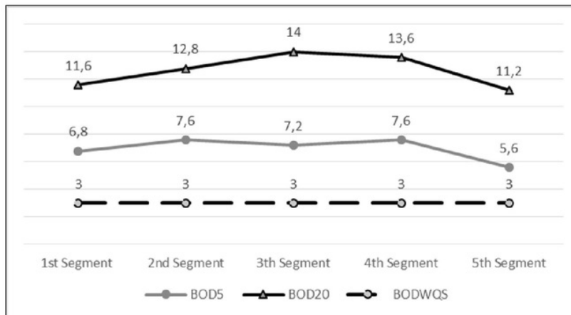
Figure 2 Comparison of BOD 5 , BOD 20 and BOD WQS
