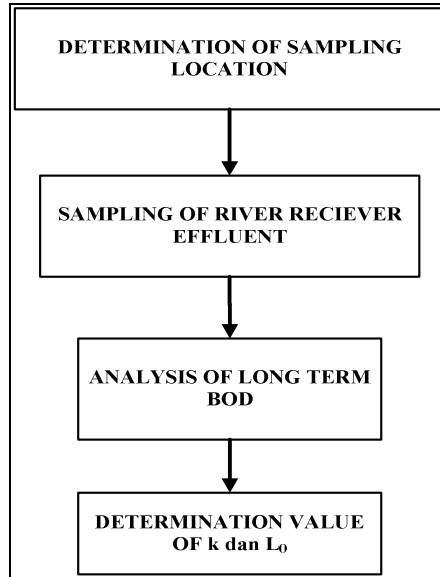
Figure 1. Flow Diagram Of Determination Deoxygenation Rate Carbon
