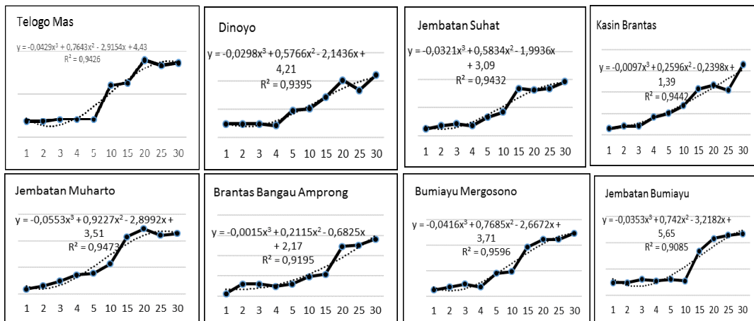
Figure 3. Trend of Long Term BOD Analysis
