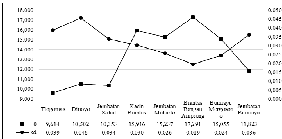
Figure 6. Fluctuation of k and L_0 Value
