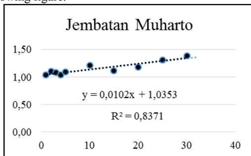
Figure 5. Plot (t/y)^{1/3} VS t
