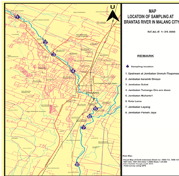
Figure 2 Segmentation of the River
