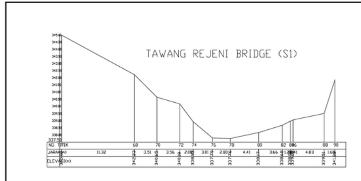
Figure 9. Cross section profile of the river at Sampling Point S1
