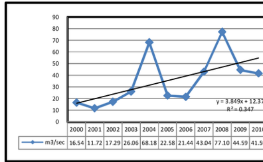
Figure 6. Annual Average Flows of Lesti River (Upstream-Tawangrejeni)
