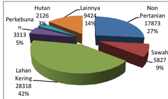
Figure 4. Land Use of Lesti River Area
