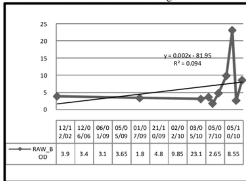
Figure 15. Trend of BOD Concentration (mg/l)
