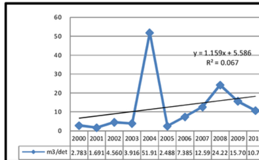
Figure 7. Annual Minimal Flows of Lesti River (Upstream-Tawangrejeni)
