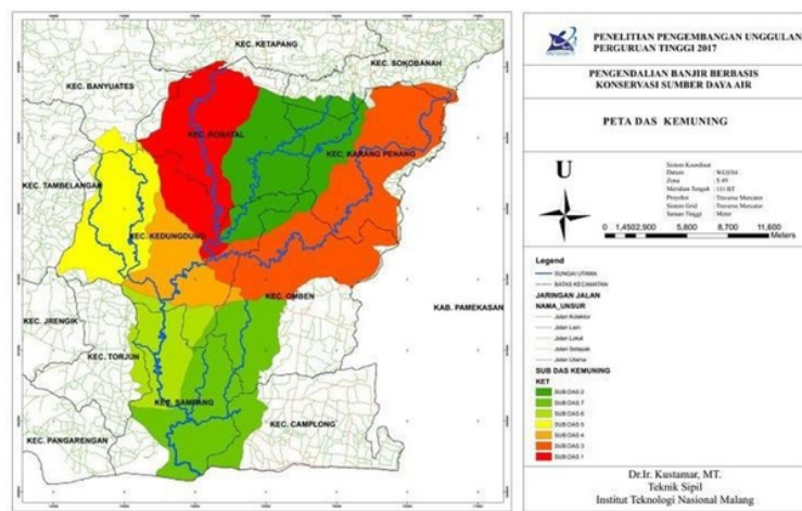
Figure 2. Kemuning Watershed
