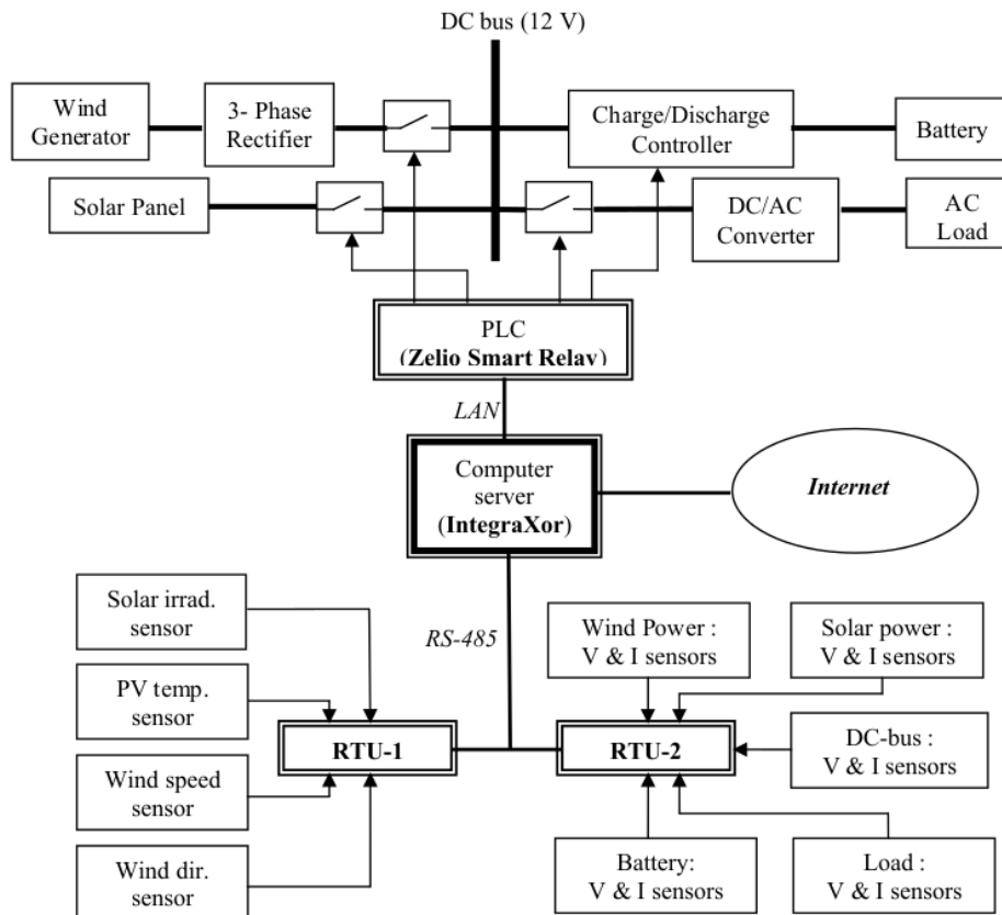
4 Figure 2. Hardware configuration of SCADA system
