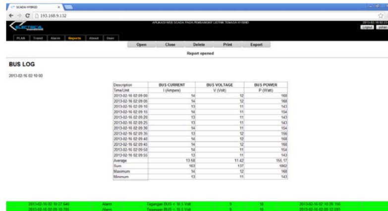
Figure 10. SCADA report display of the DC-bus
