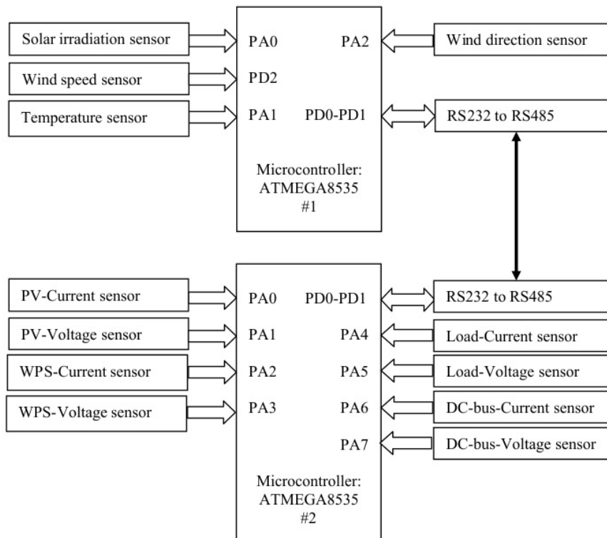
Figure 4. Block diagram of RTUs and sensor modules.
