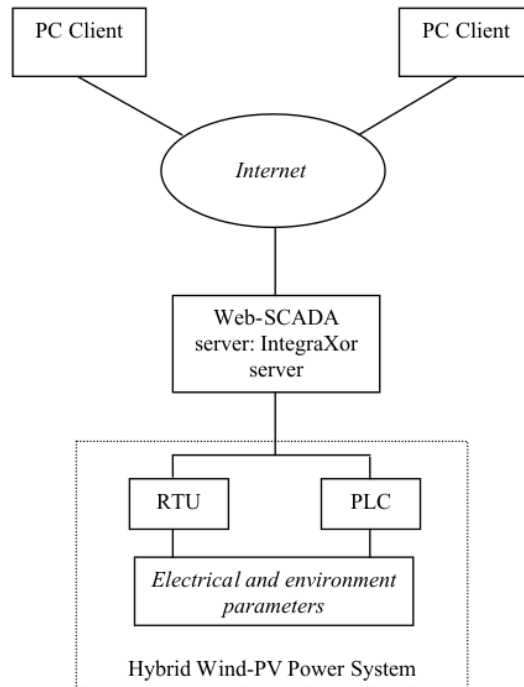
Figure 1. SCADA architecture.
