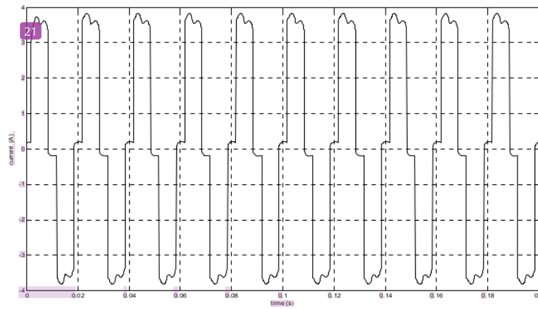
Figure 5 Source current for rectifier with inductive load
