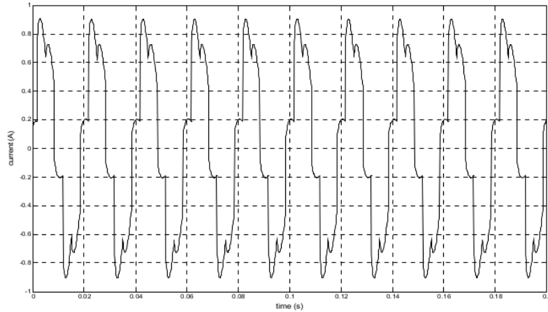
Figure 4 Source current for rectifier with resistive load
