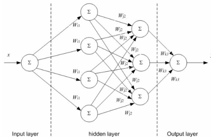
Figure 1 Architecture of MLPNN
