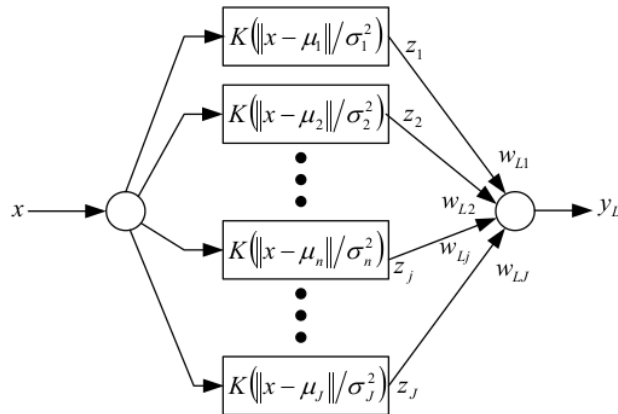
Figure 2 Typical structure of RBFNN
