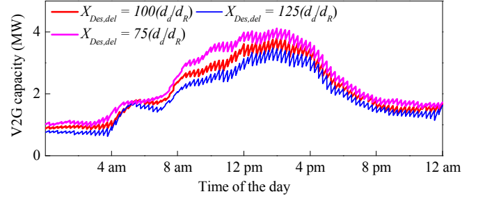
Fig. 6. Diurnal V2G capacities of UQ parking lots for various X_{Des,del} .
