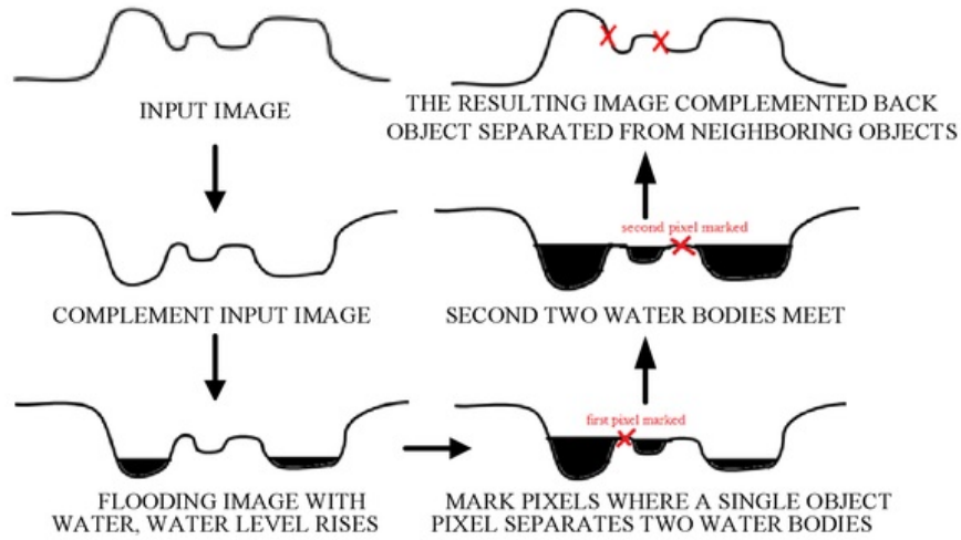
Figure 4. Watershed process
