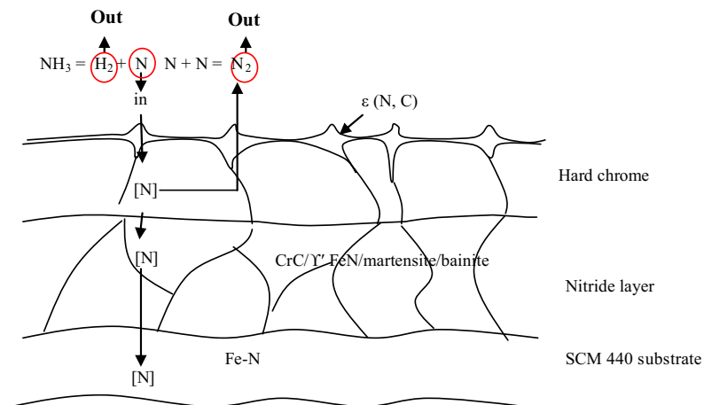
Figure 12 The mechanism illustration of layer \epsilon and \gamma' area formation at diffusion stage in muffle reactor (see online version for colours)
