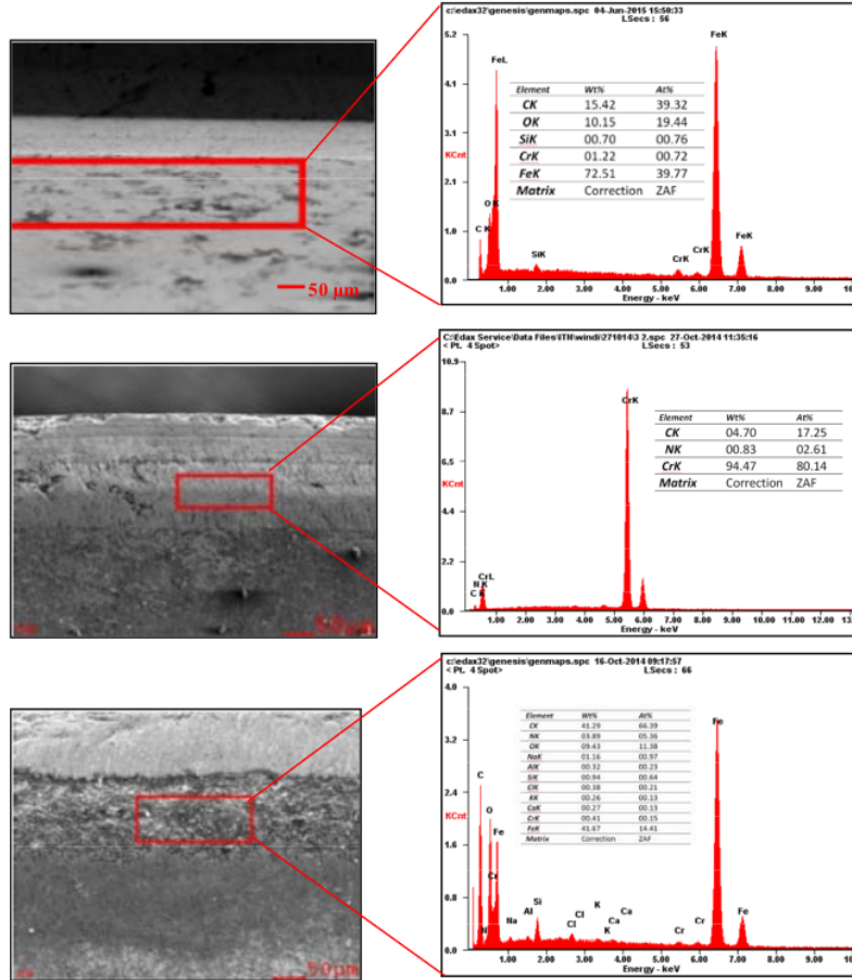
Figure 9 The result of EDAX sensation composition test on chromium plated steel, (a) without treatment (b) nitriding treatment of nitrogen diffusion media (c) nitriding treatment of nitrogen gasless nitrogen media (see online version for colours)
