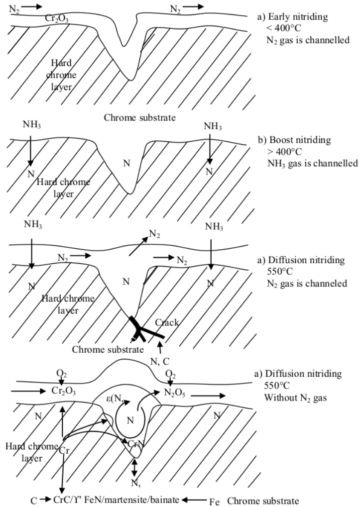
Figure 13 The sensitisation phenomena on hard chrome plated steel during the nitriding process
