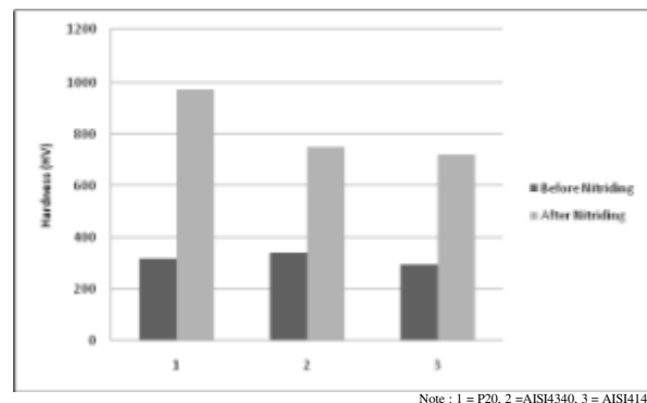
Fig 4. Hardness of some tool steels before and after nitriding process
