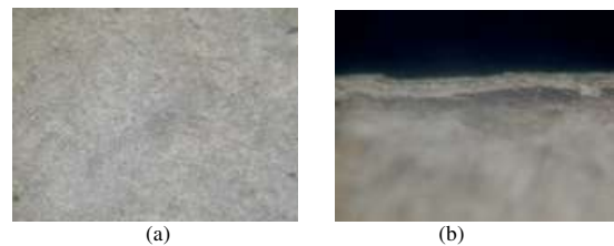
Fig 3. AISI 4140 Microstructure (250x) a) before, b) after nitriding
