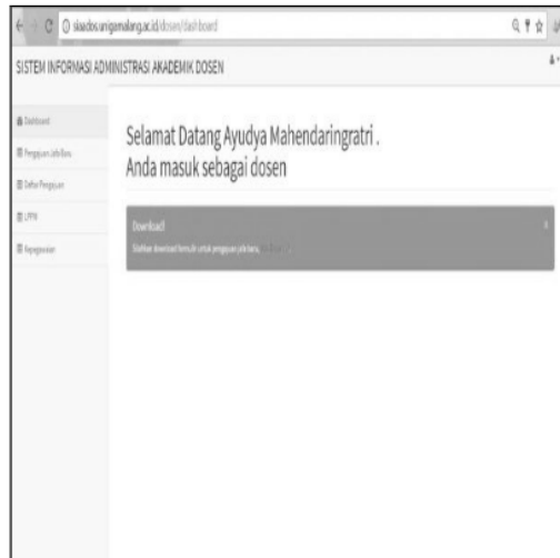
Gambar 4. User Interface
