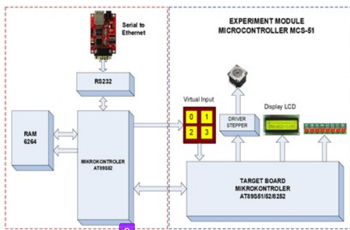
Figure 7. EWS Block Diagram and Experiment Module
