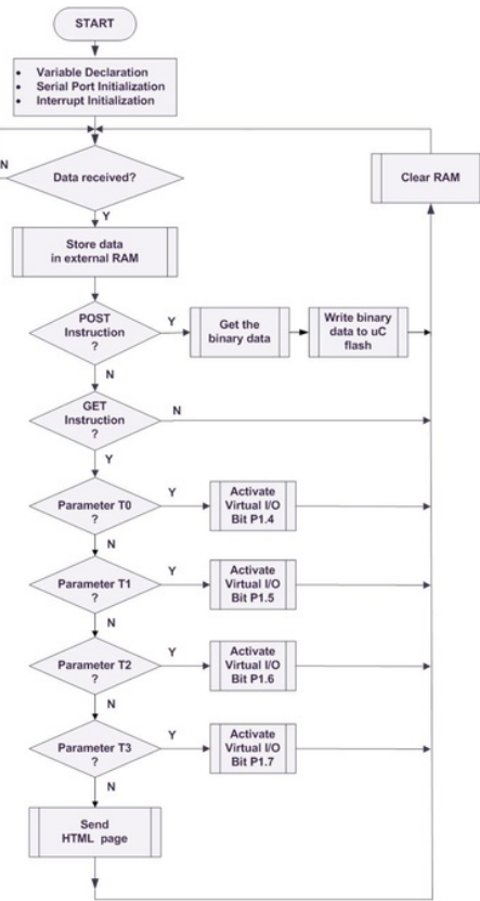
Figure 8. Embedded Web Server Flow Chart
