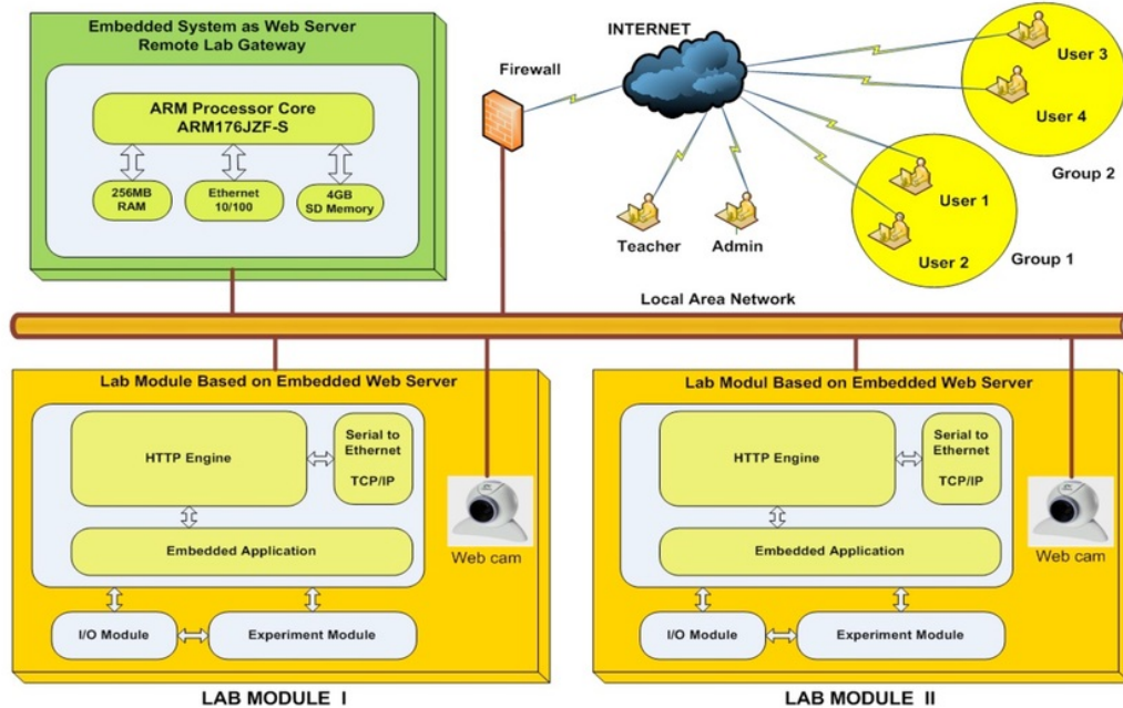
Figure 1. Remote Lab Architecture
