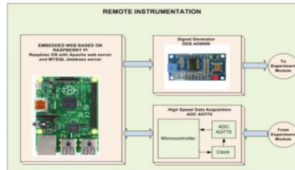
Gambar 2. Diagram sistem Instrumentasi Remote
