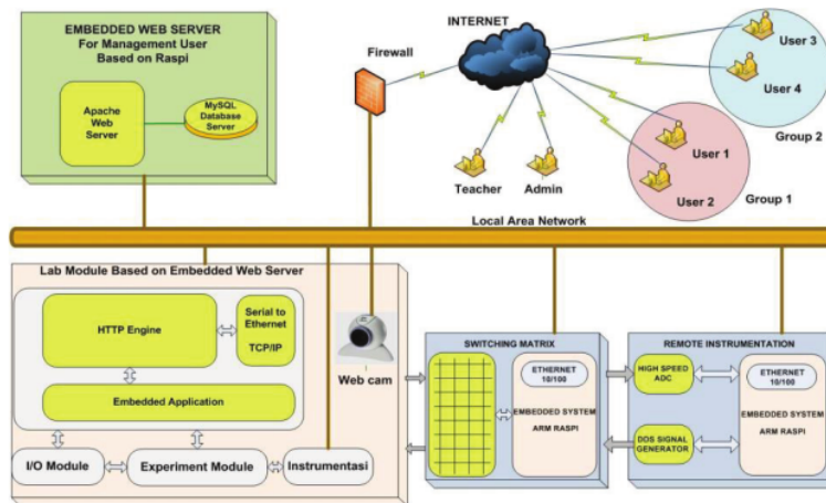
Gambar 1. Diagram Arsitektur Laboratorium Remote
