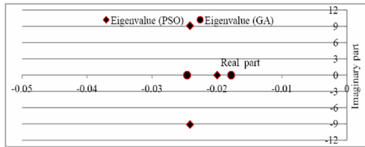
Figure 7 Eigenvalues after optimal placement of UPFC in IEEE 14-bus system using both the PSO and GA techniques (see online version for colours)
