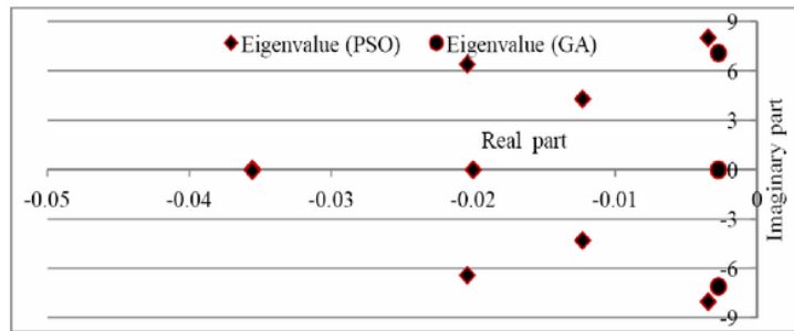
Figure 16 Eigenvalue after optimal placement using SVC in Java-Bali 24-bus Indonesian system using both the PSO and GA techniques (see online version for colours)
