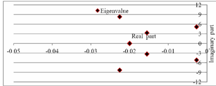
Figure 12 Eigenvalue after optimal placement of UPFC in IEEE 30-bus system using the PSO technique (see online version for colours)
