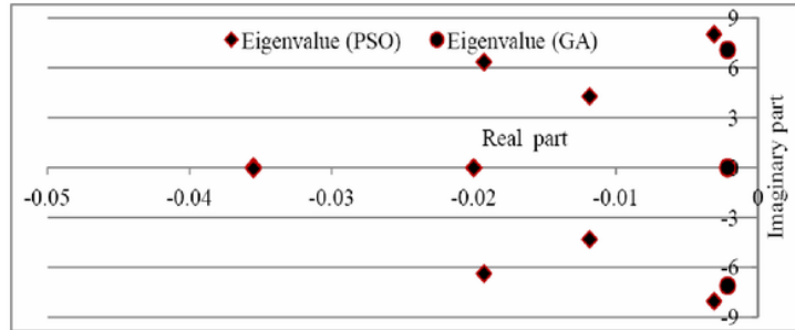
Figure 15 Eigenvalue after optimal placement using TCSC in Java-Bali 24-bus Indonesian system using both the PSO and GA techniques (see online version for colours)
