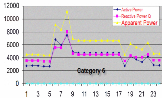
Figure 7. Typical load duration curves category 6.
