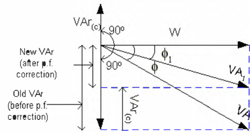
Figure 1. Power factor correction phasor diagram.
