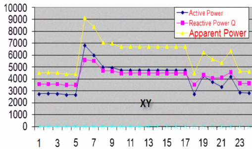
Figure 9. Typical load duration curves XY
