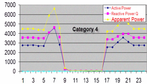
Figure 5. Typical load duration curves category 4.
