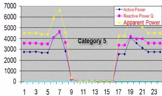
Figure 6. Typical load duration curves category 5.
