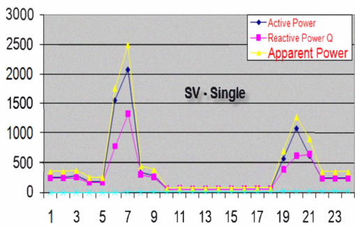
Figure 10. Typical load duration curves SV-single.
