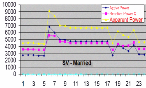
Figure 8. Typical load duration curves SV-married.
