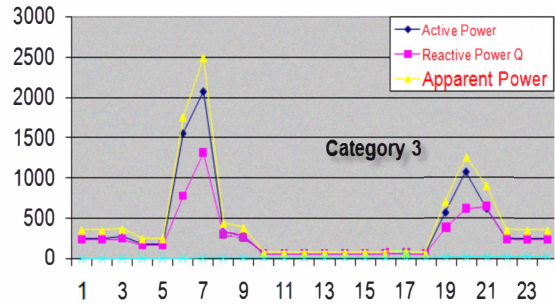
Figure 4. Typical load duration curves category 3
