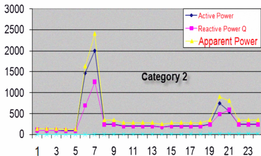
Figure 3. Typical load duration curves category 2.
