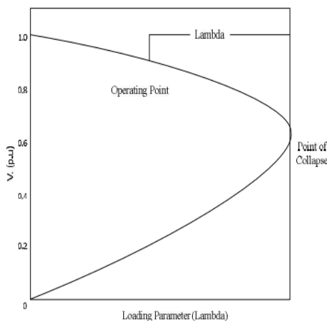
Gambar 1. Maximum Loadability Parameter \lambda_{max} = \lambda + 1 .
