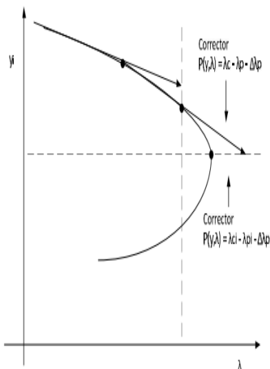
Gambar 4. Continuation Power Flow: Tahap Koreksi [7]
