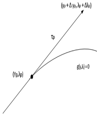
Gambar 2. Continuation Power Flow: Predictor Step. [7]
