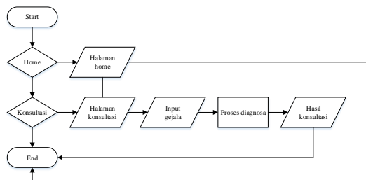
Gambar 3.2 Flowchart user
