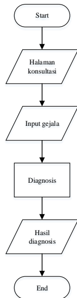
Gambar 3.1 Flowchart sistem
