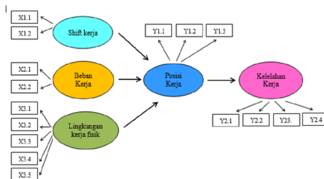
Figure 1. PLS Model Flow Chart
