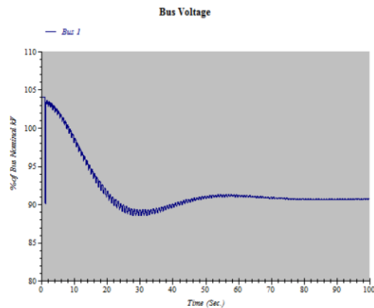
Figure 5: Voltage response when G3 out from system (t=1,1 s)
