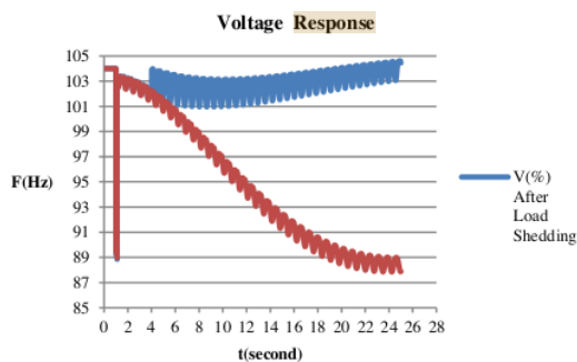
Figure 7: Voltage response before and after load shedding
