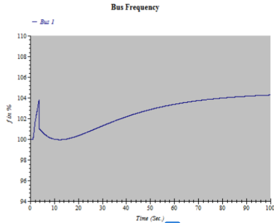
Figure 2: Frequency response during 3 phase short circuit ( t=1 s)
