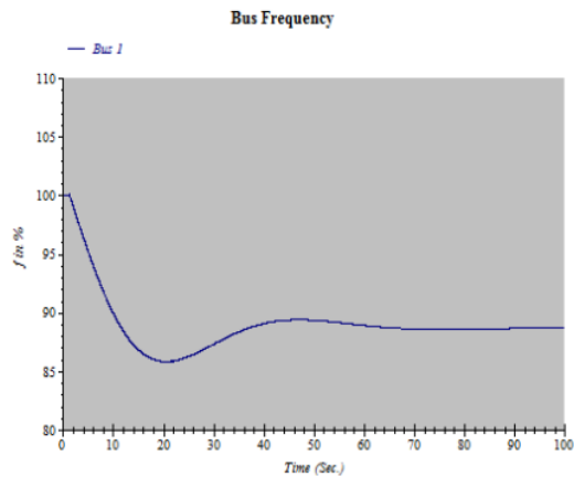
Figure 4: Frequency response when G3 out from system (t=1,1 s)
