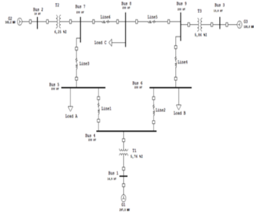
Figure 1: IEEE 9 Bus system
