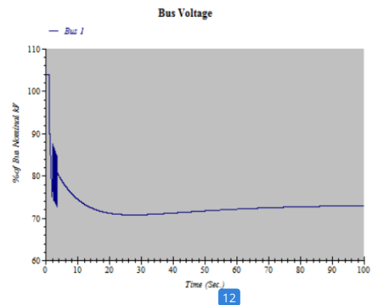
Figure 3: Voltage response during 3 phase short circuit ( t=1 s)
