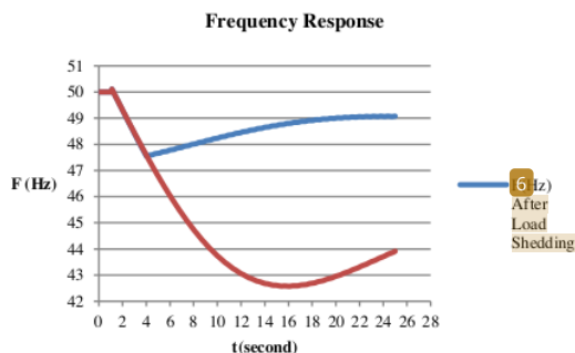
Figure 6: Frequency response before and after load shedding
