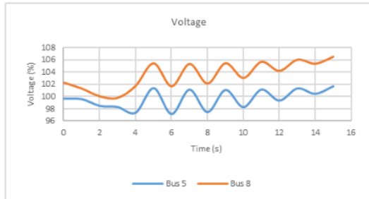
Fig. 9. Voltage Increase at Bus 5 and 8
