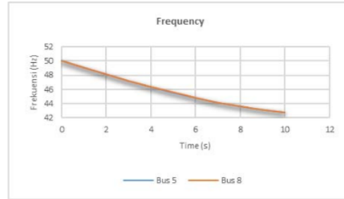
Fig. 4. Frequency Decrease at Bus 5 and 8
