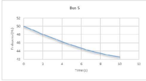
Fig. 2. Frequency Decrease at Bus 5
