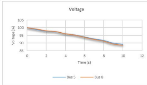
Fig. 5. Voltage Decrease at Bus 5 and 8
