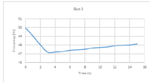
Fig. 6. Frequency Increase at bus 5
