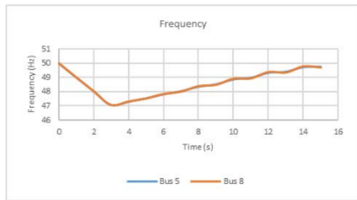
Fig. 8. Frequency Increase at Bus 5 and 8
