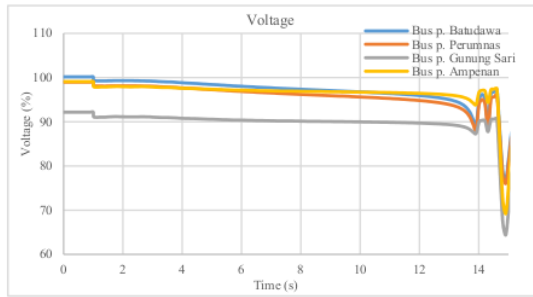
Fig. 7. Plotting voltage on bus feeder GI Ampenan
