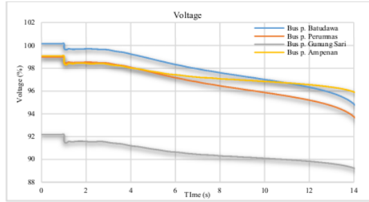
Fig. 3. Plotting voltage at feeder GI Ampanan
