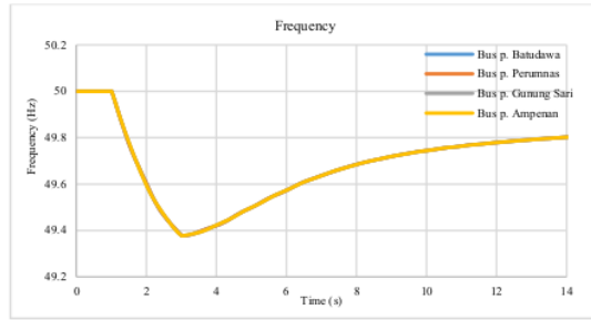
Fig. 4. Frequency on bus feeder GI Ampanan after load shedding.
