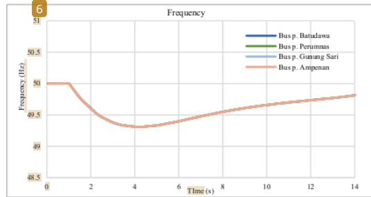
Fig. 2. Response frequency on bus feeder GI Ampanan
