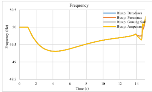
Fig. 6. Frequency feeder GI Ampenan
