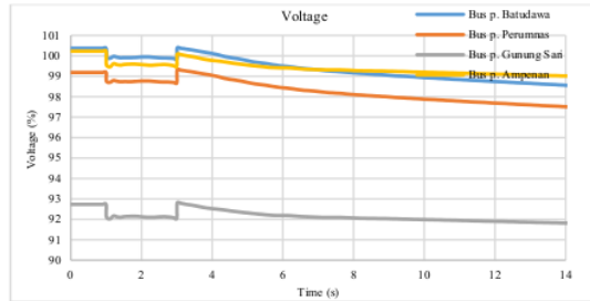
Fig. 5. Voltage profile after Load Shedding on GI Ampanan
